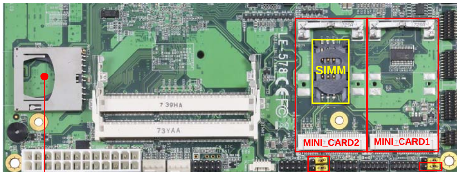
SD Slot
