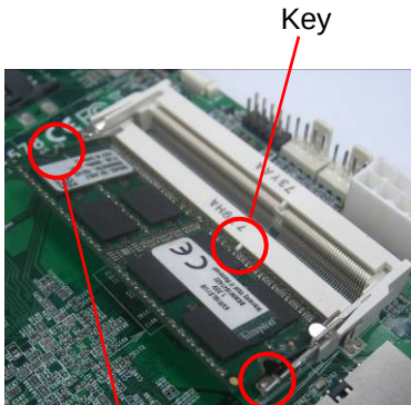
Mounting notch
