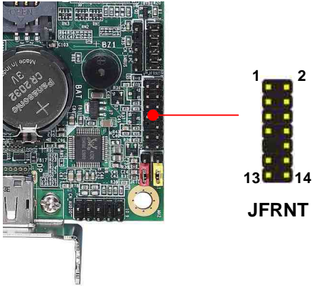
JFRNT: Front panel switch and indicator 14-pin header (Pitch 2.54mm)
